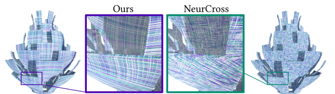
Fig. 9. Comparisons with NeurCross near features. Our approach enhances curvature alignment by reweighting the alignment energy based on principal curvature difference [Zhuang et al. 2014], typically leading to better feature preservation compared to NeurCross.
