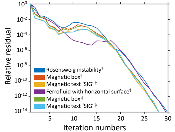
Fig. 5. Relative residuals of magnetic fields as the iteration number increases in our multi-grid solver for different configurations. \dagger denotes the uniform external field while \ddagger denotes the external field induced by a magnet.
