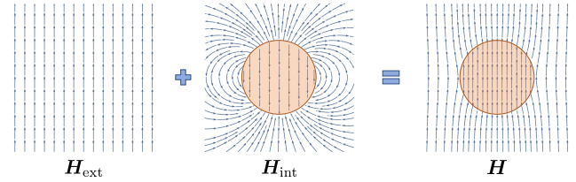
Fig. 3. An example of magnetization and induction. A sphere in a uniform magnetic field ( \mathbf{H}_{\text{ext}} ) is magnetized and produces an induced field ( \mathbf{H}_{\text{int}} ), which will further lead to a synthesized field ( \mathbf{H} ).
